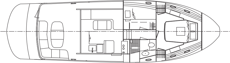
2 cabin floor plan
